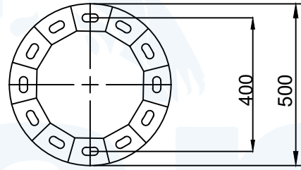
BASE PLATE t=22 mm
