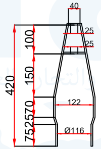
A CLAMP
