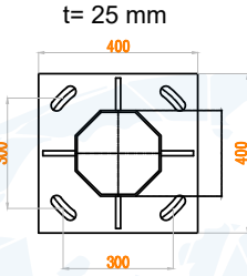
BASE PLATE C-C SECTION
