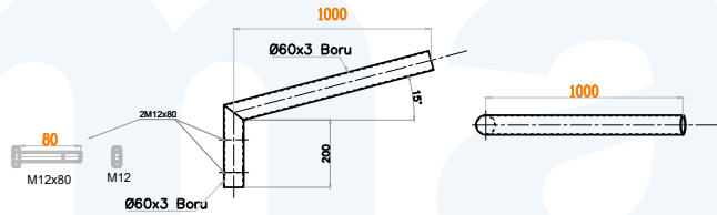
SINGLE BRACKET ARM DETAIL
