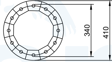
BASE PLATE t=20 mm
