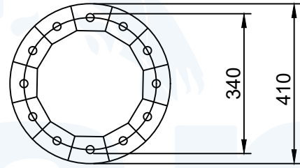
BASE PLATE t=20 mm
